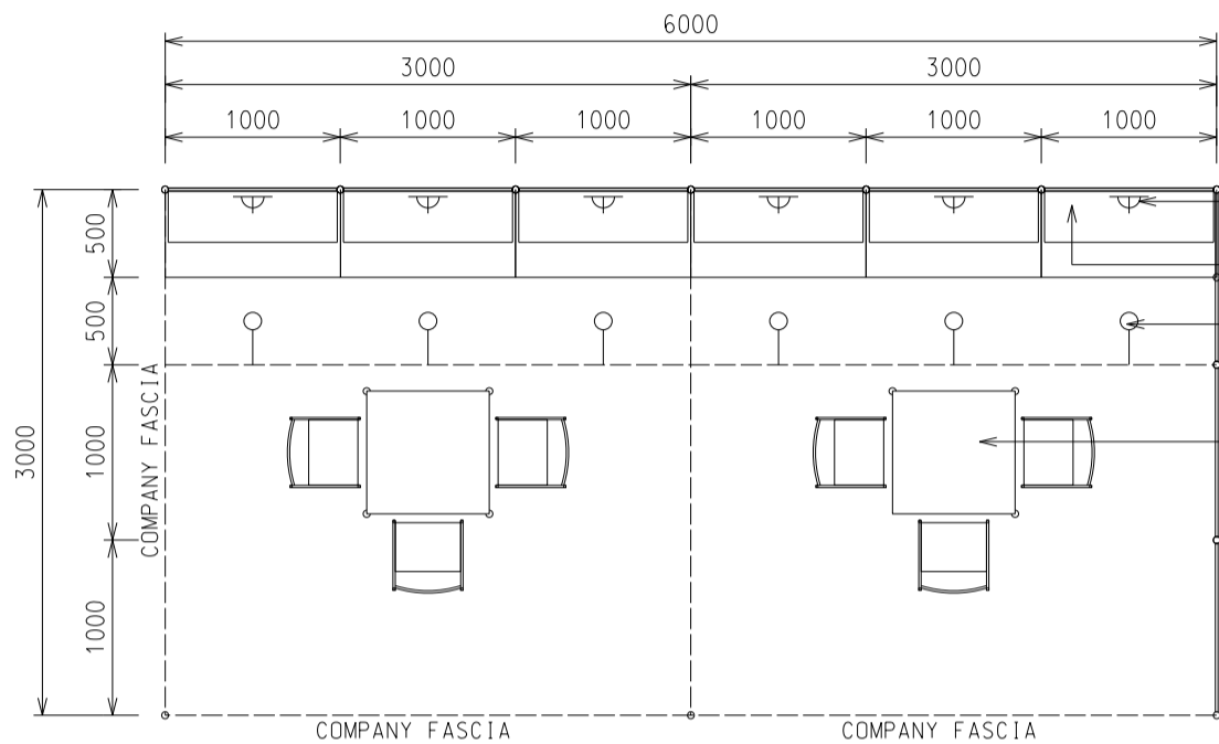
PLAN 6M(W) X 3M(D) X 2.5M(H) Left Corner Booth A
